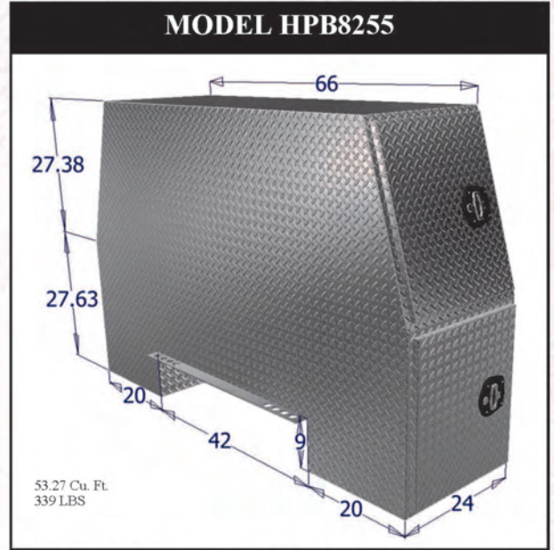
2 Fixed Shelves (.125 Thick Smooth Aluminum)
