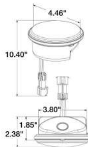
27270C LED Headlight
