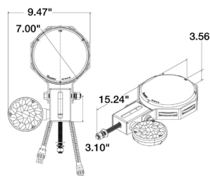
80990 Kit Includes 80988 light, 80989 light, 80988 harness
