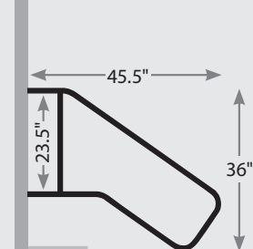
AC-500L with a 7" Rise and 11" Run Step
