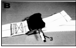
Figure B: Position the plastic cover on top of the loop and insert the metal retainer [3] through the guides of the plastic cover and the strap loop.
