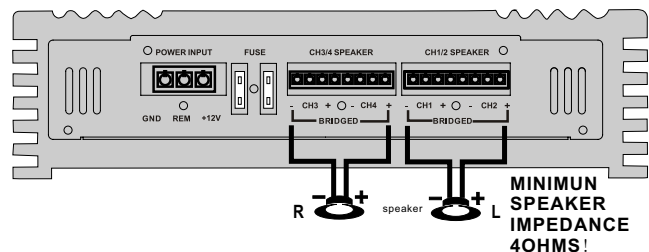
Bridged Dual Mono Output Mode
