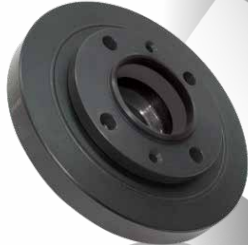
PN 2328951 - FORD 221-260, 289-351W, 302B, 1963-69, Early Model SB Ford, Spacer Pictured Not Required for All Models; Available Separately (See Page 60)
