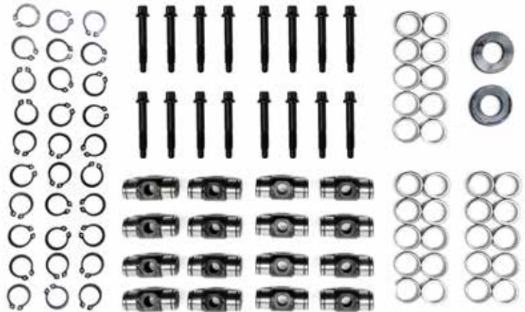
PN 1213462 GM LS Series Roller Bearing Fulcrum Upgrade Kit
