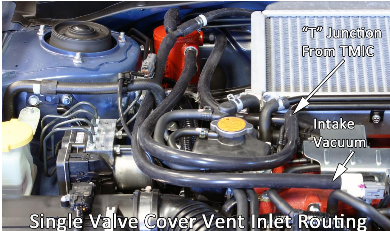
The above setup shows a simple setup that uses the OEM valve cover vent piping that bolts to the top mounted intercooler.
