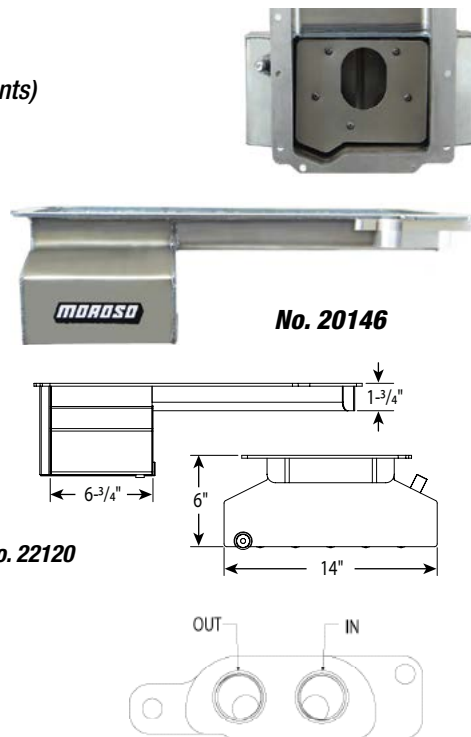
No. 23688 Remote Oil Filter Adapter, GM LS Series, Included with No. 20146
