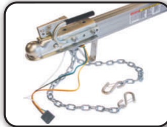
2" Receiver with Lift Handle and Four Pin Connector
