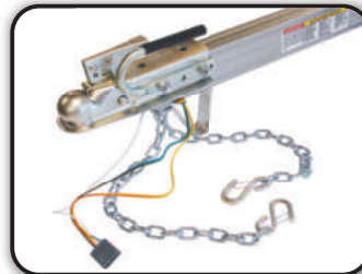
2" Receiver with Lift Handle and Four Pin Connector
