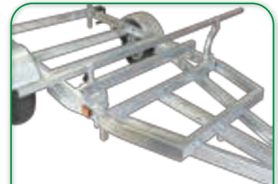
86" Steel Load Bars with 3.5" x 1.5" C-Channel Construction
