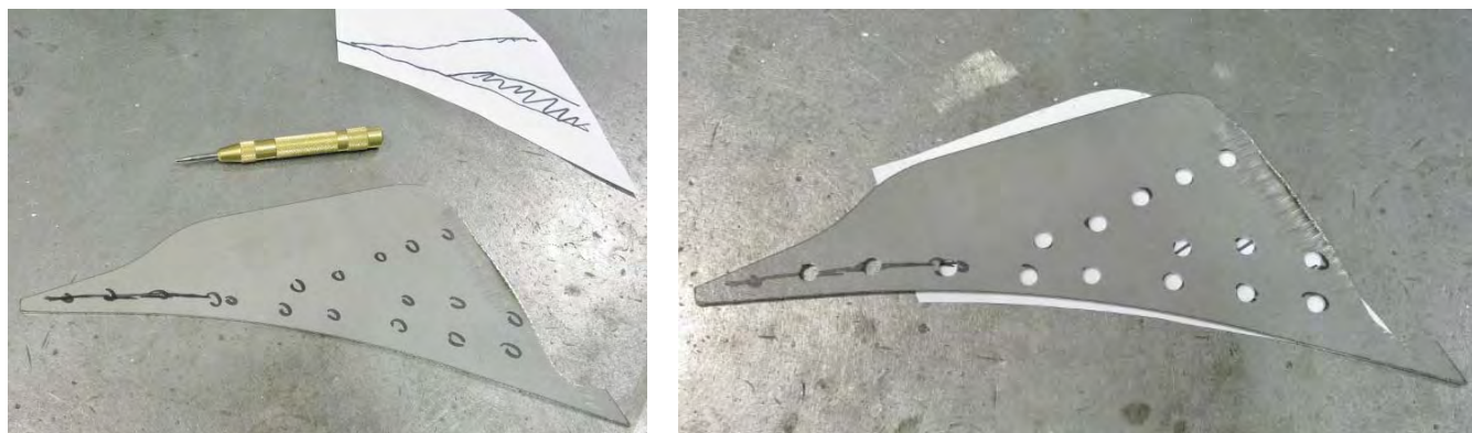
Figure 34 - Drill or Punch Plug Weld Holes
