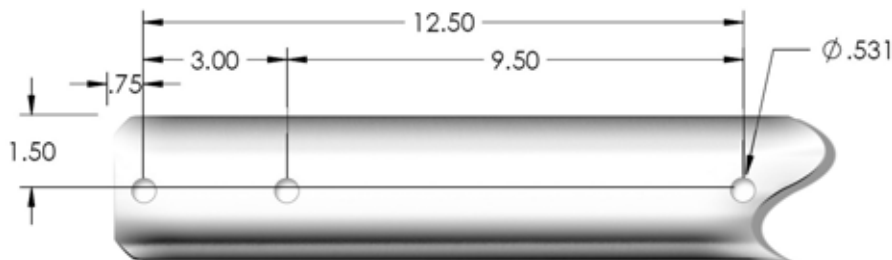
3 Hole Standard
