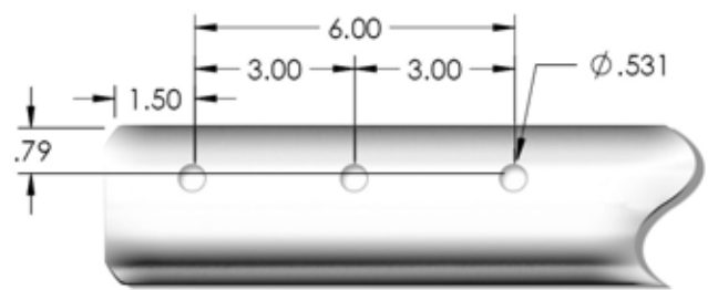
3 Hole Straight
