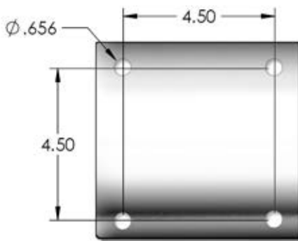
Flat Mount
