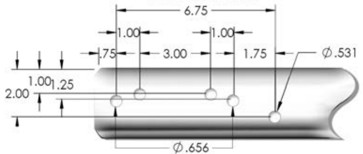
5 Hole Standard
