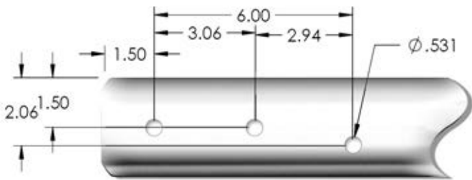
3 Hole
