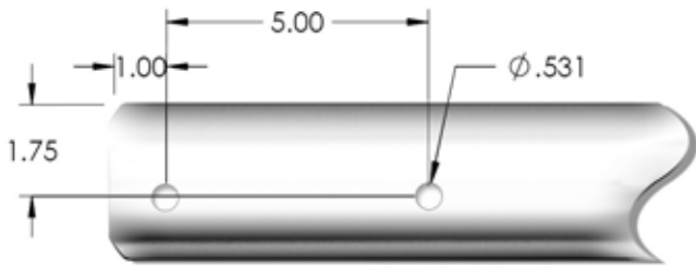
2 Hole Standard
