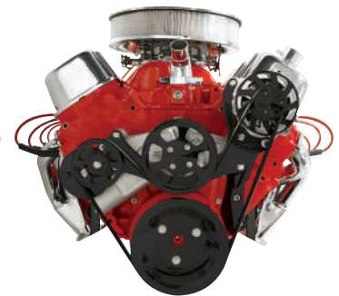
Without AC Without Power Steering BLK14125
