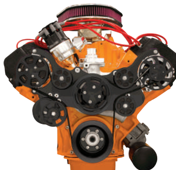
With AC Without Power Steering BLK14820
