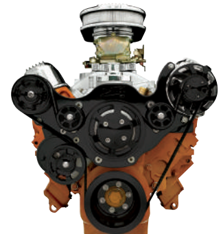
Without AC Without Power Steering BLK13825
