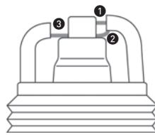
Schematic diagram of spark paths. 1 Air sparks 2 Auxiliary surface gap sparks 3 Air.
