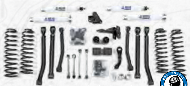
Kit shown with optional forged flex end lower control arms (Standard kit uses fixed lower arms)
