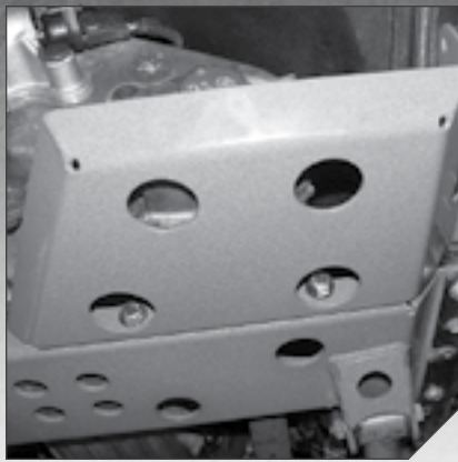
#124656 - Optional Transfer Case Skid Plate. Will only work with NP231. Shown in gray, available in black only
