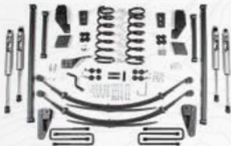
#248H - 5" Long Arm kit shown w/ optional FOX 2.0 shocks
