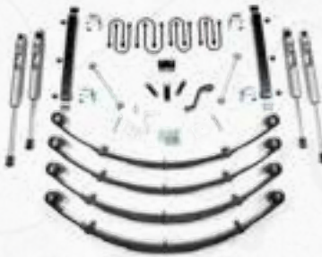
#409H - 3.5" kit shown w/ optional FOX 2.0 shocks
