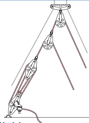
16:1 Split backstay
