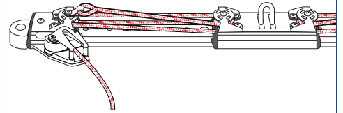
4:1 Traveller cleats on end
