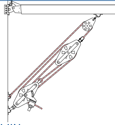
8:1 Cascaded kicker
