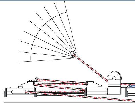
4:1 Genoa car
