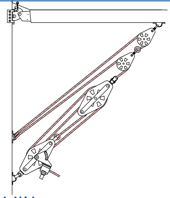
16:1 Cascaded kicker
