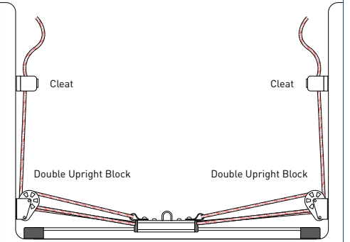
3:1 Remote cleat
