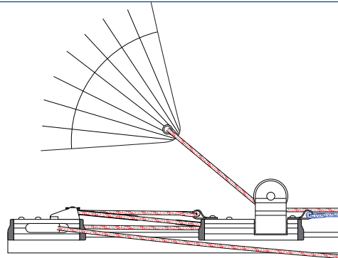
3:1 Genoa car
