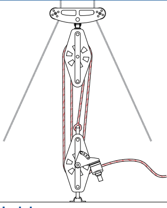
4:1 Split backstay
