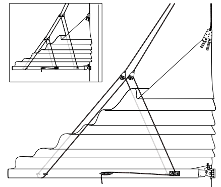
Lazy jacks
