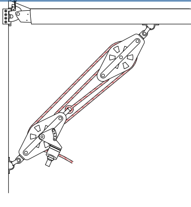
4:1 Split backstay
