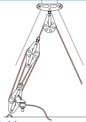
8:1 Split backstay
