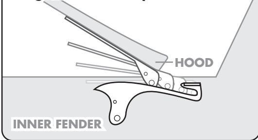
Diagram B - Closeup Runner/Slider
