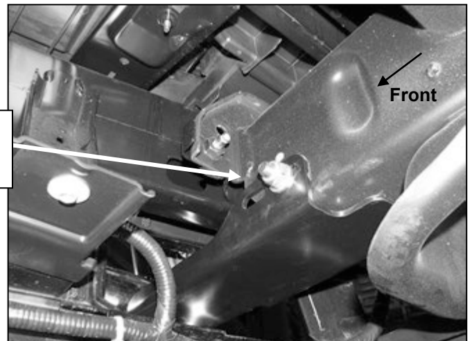
(Fig 7B) Passenger Bracket installed in "forward" position to move Bull Bar away from bumper
