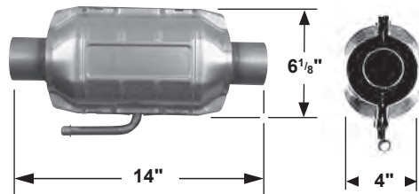
Oval - w/o Air Tube
