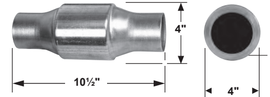
Spun Body one-piece design Round - w/o Air Tube
