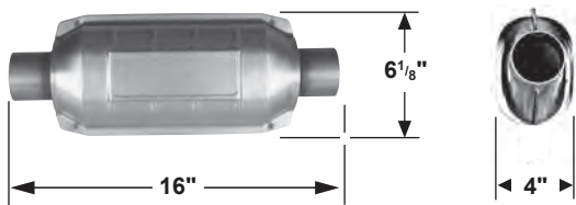
Oval - w/o Air Tube
