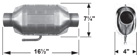
Oval - w/Air Tube
