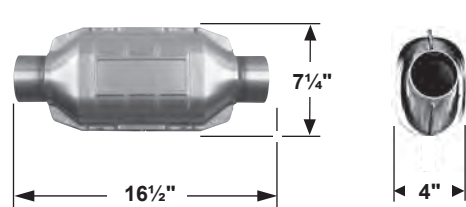
Oval - w/o Air Tube
