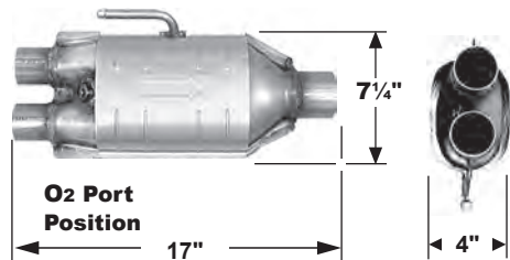
Oval - w/Air Tube
