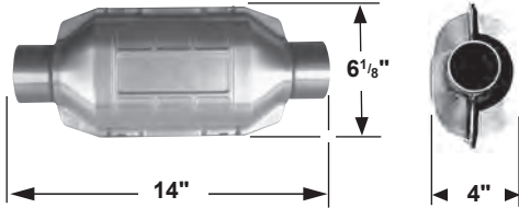
Round - w/o Air Tube
