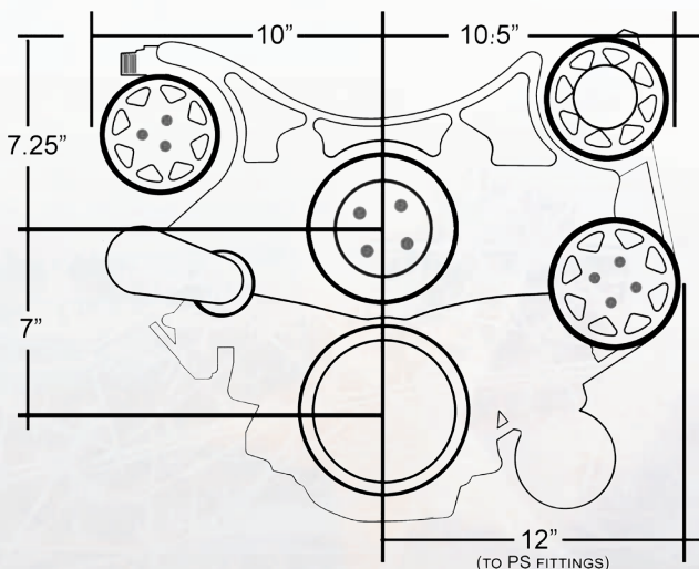
Polished - With A/C & With Power Steering FDS-440-101
