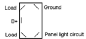
DS-1817 Toggle Switch
