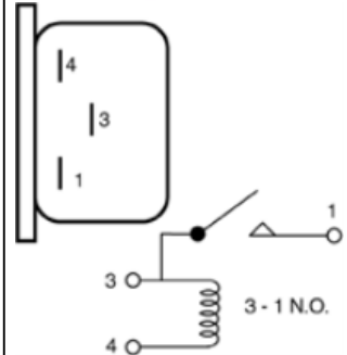
HR-118 Horn Relay
