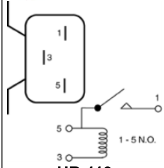
HR-119 Horn Relay
