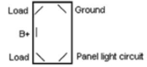
DS-1815 Toggle Switch
