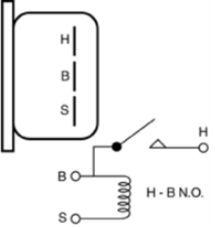
HR-106 Horn Relay
