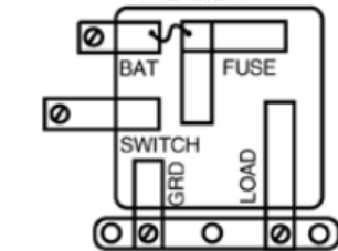
LR-32 Multi-Function Relay 1116969; 6D6306 Cadillac..... 1967 - 1965
