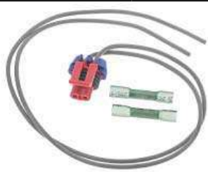
S-1350 A/C Cycling Switch Connector 13585860; 12101858
