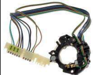
DS-1466 Turn Signal Switch 01995970; 1995970 Chevrolet ..... 1996 - 1994 GMC ..... 1994
