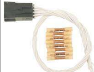
S-1227 A/C Control Module Connector 12125682; 12089648; 15306155; 15306023
