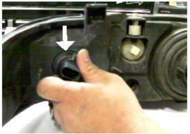
10. Remove the signal socket from the OEM headlight
