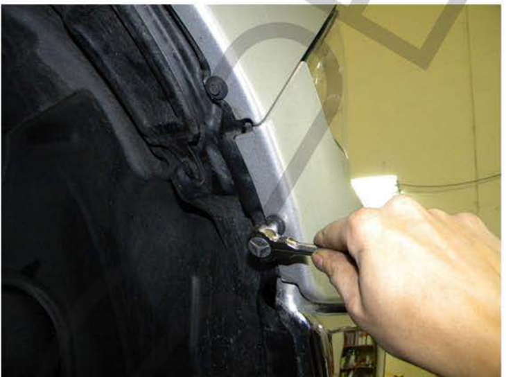
27. Tighten the (2) 8mm bolts Please repeat the steps in order from 1 to 27 for the opposite side
