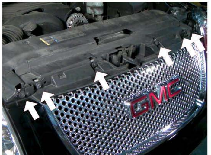
16. Install six bolts for the top front grill
