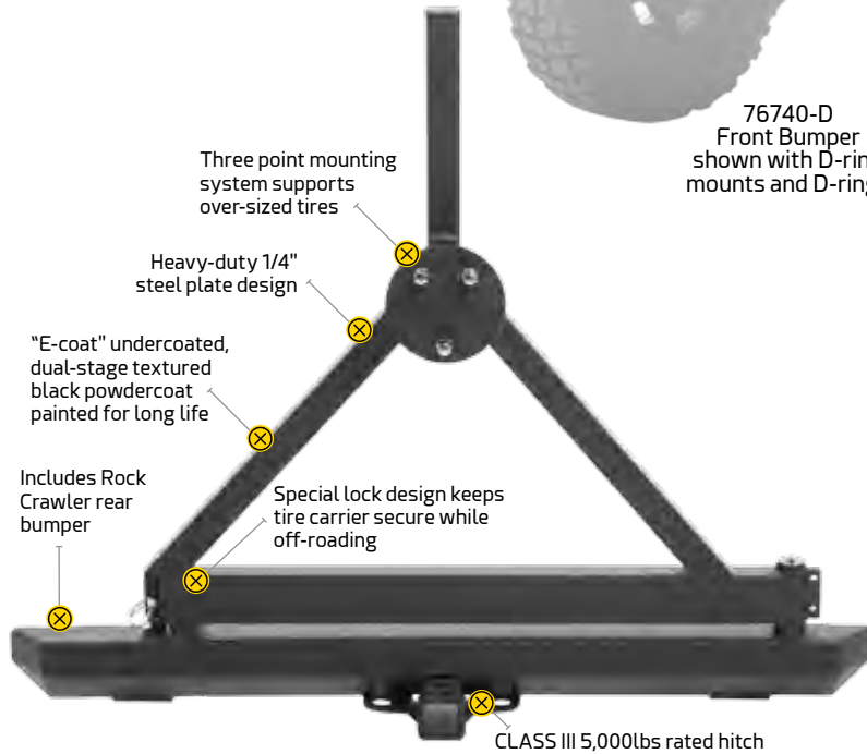
76751-D Shown with Tire Carrier, D-Ring mounts & D-rings
