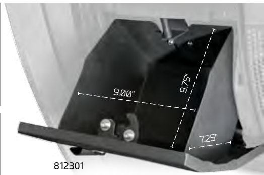
Mounts into O.E. holes
