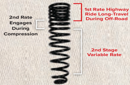
2-STAGE VARIABLE RATE REAR COILS
