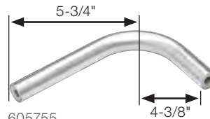
605755 (10" before being bent)
