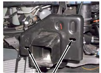
Remove the bumper mounting nuts from behind the frame flange
