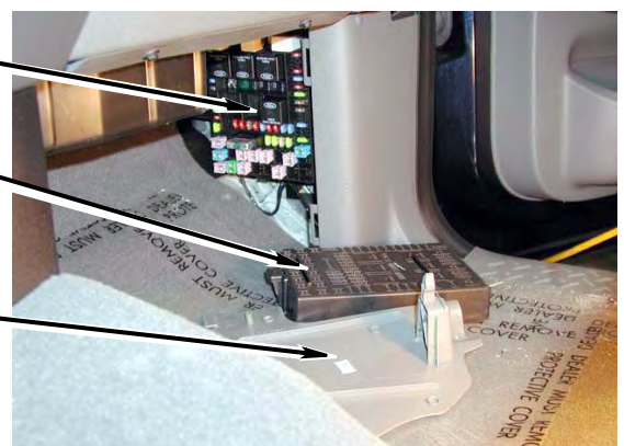
Fuse Panel Cover
