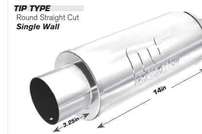
STREET PART# 14822
