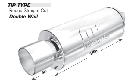
STREET PART# 14817
