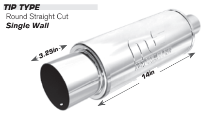
STREET PART# 14857
