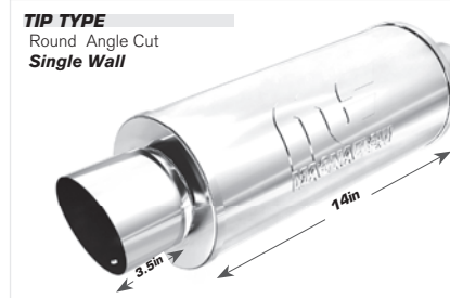
STREET PART# 14823
