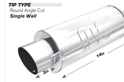
STREET PART# 14821
