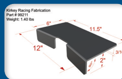
Rear Seat Mount #99211
