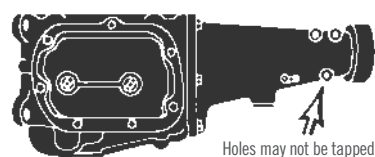
SAGINAW (343) 7-bolt side cover; first-gear synchronized CAUTION: This transmission closely resembles 351 Muncie Holes may not be tapped
