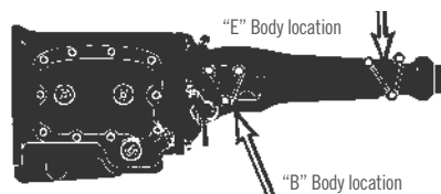
NEW PROCESS, MOPAR (423) 10-bolt side cover "E" Body location "B" Body location
