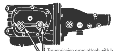
MUNCIE M-22 (453) G.M. 7-bolt side cover 1970, 454 Chevelle Transmission arms attach with bolt
