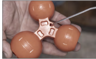
Built-in safety points allow the ball to break off when forcefully tampered with, leaving the ball in the coupler and blocking hookup
