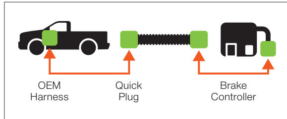
Quick plug equipped for fast, easy installation (excluding Echo®)
