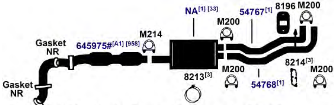
[A1] Combination Front and Rear Converter, 2 To 1 Replacement. Only Defective Converters May Be Replaced.
