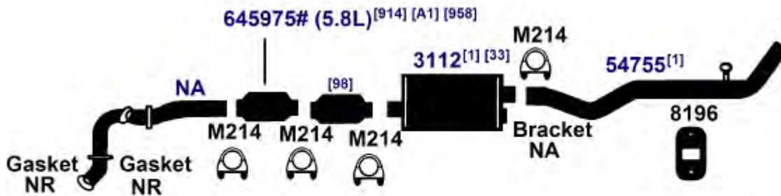
[A1] Combination Front and Rear Converter, 2 To 1 Replacement. Only Defective Converters May Be Replaced.
