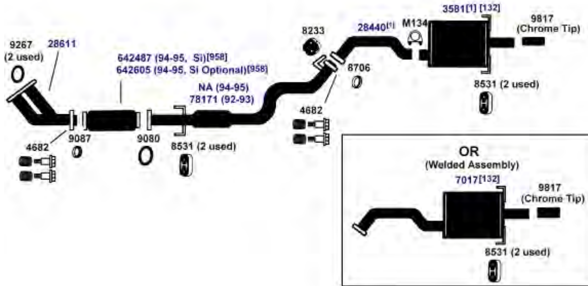
DIRECT FIT MSL/MAXIMUM Muffler... Split System- 700169
