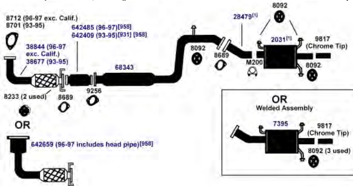
DIRECT FIT MSL/MAXIMUM Muffler... Split System- 700155
