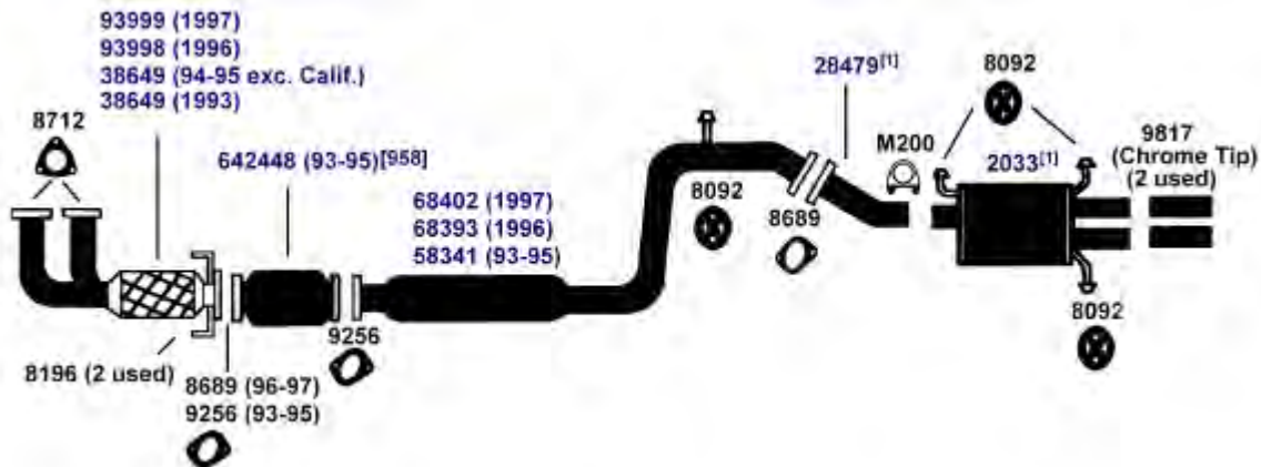
DIRECT FIT MSL/MAXIMUM Muffler... 700213
